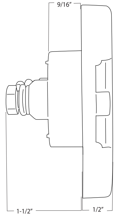
Side View Back Plate
